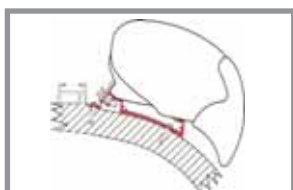
CARTHAGO CHIC 1 x 400cm bracket 18735 1 x 450cm bracket 18736 1 x 500cm bracket 18737
