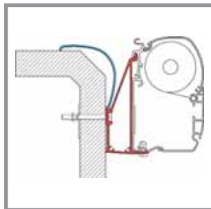
ADAPTOR SERIES 6 RAPIDO BRACKET 300CM 17965 350CM 17966 400CM 17967
